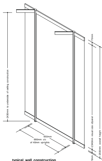
typical wall construction
